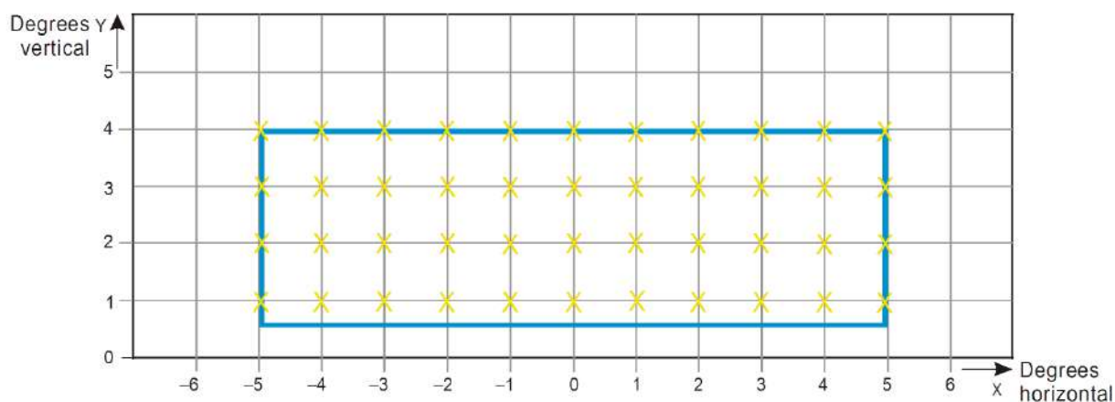
Figure A2-21. Grid points to be used for calculation of average intensity of taxiway centre line and stop bar lights
