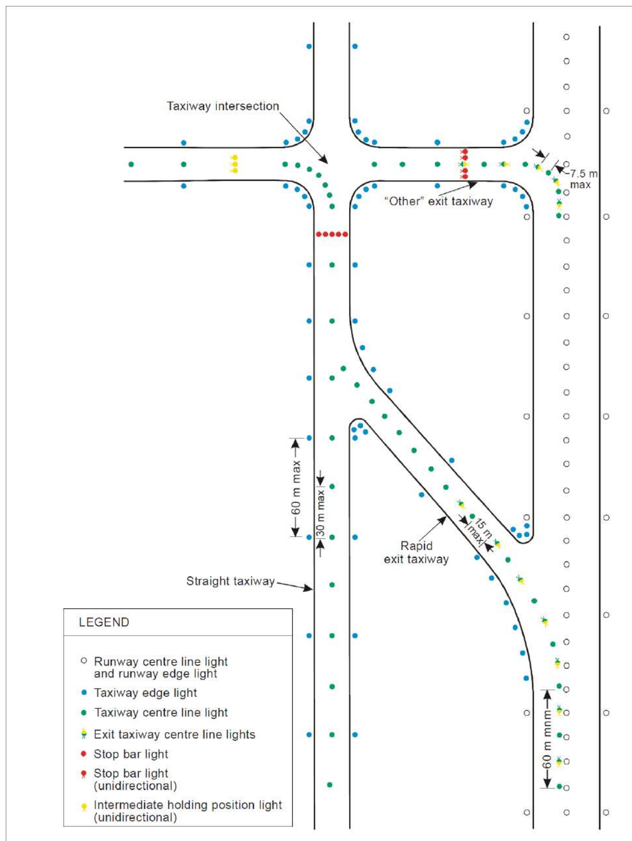
Figure 5-26. Taxiway Lighting
