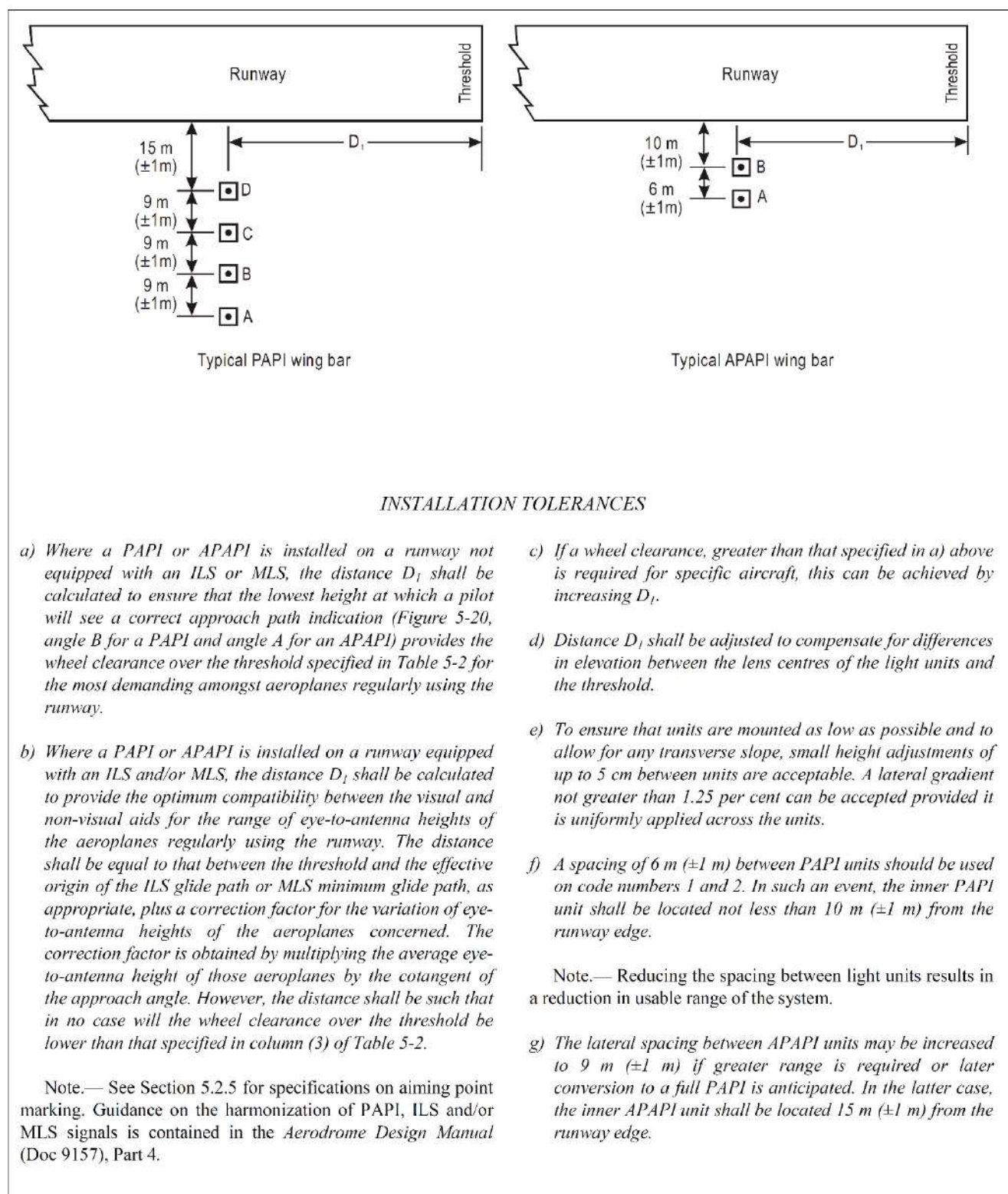
Figure 5-19. Sitting of PAPI and APAPI
