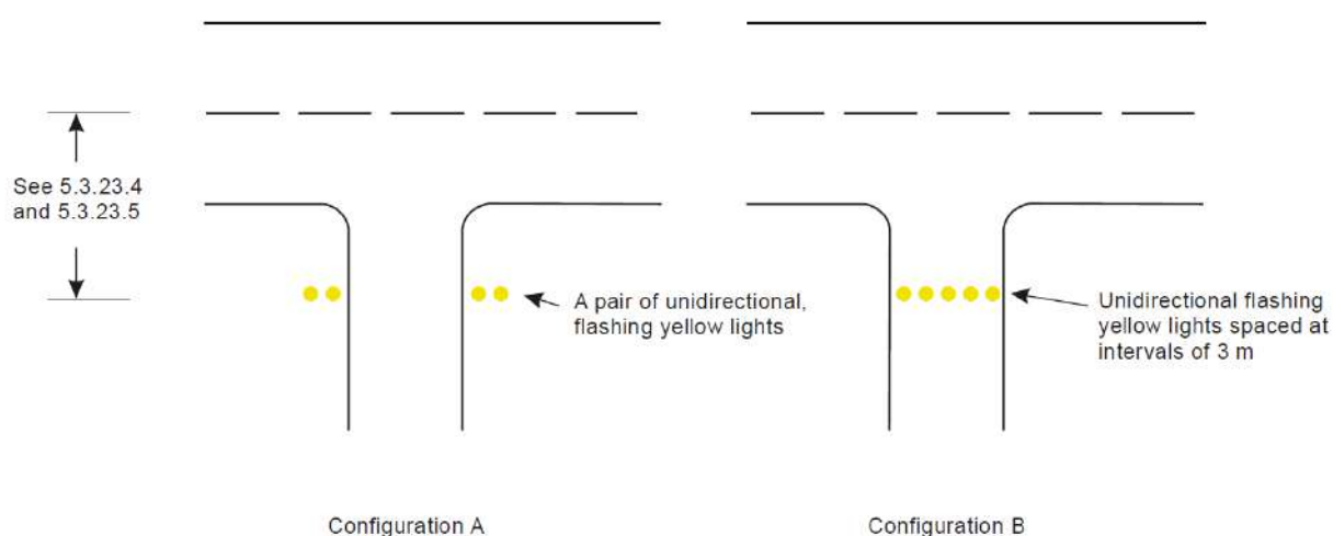
Figure 5-29. Runway Guard Light
