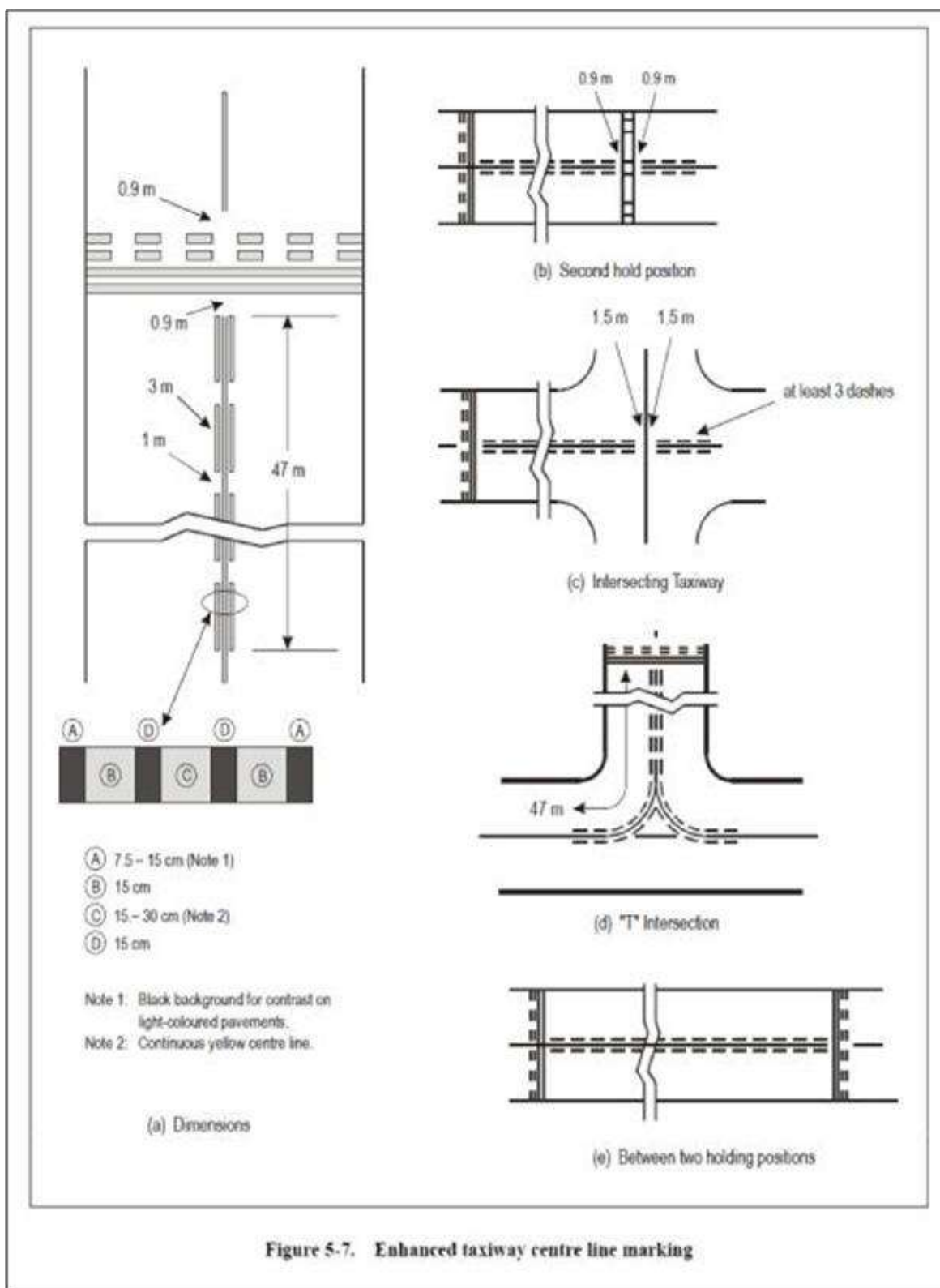
Figure 5-7. Enhanced Taxiway CentreLine Marking
