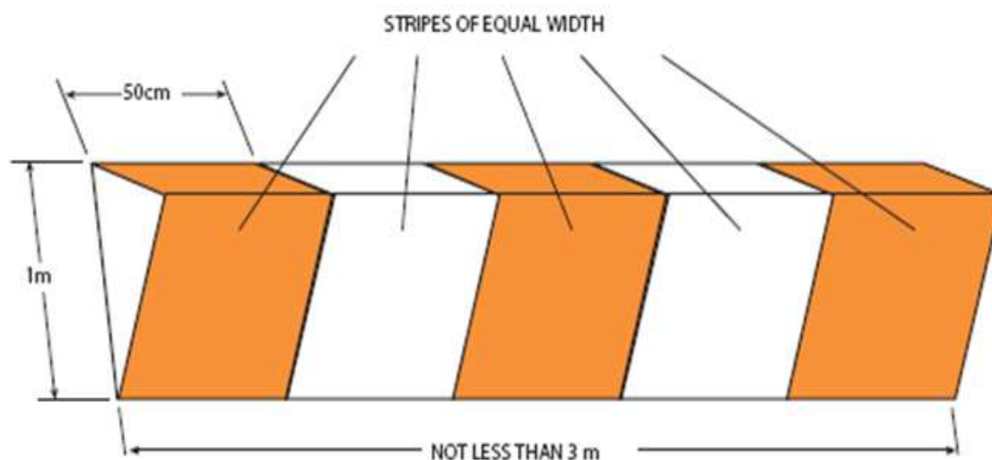
Figure 5-34. Boundary Markers
