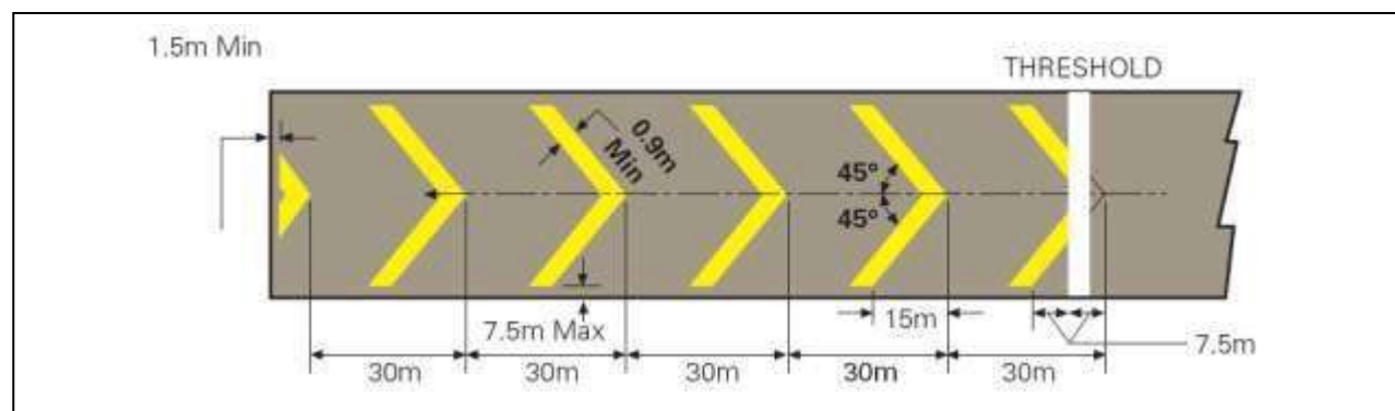
Figure 7-4. Pre-threshold marking
