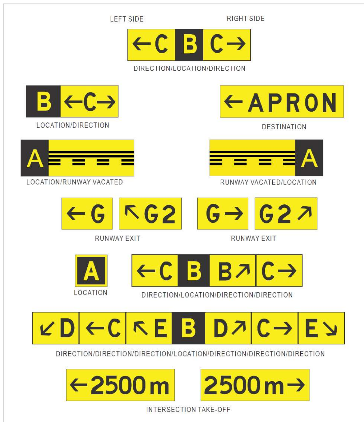
Figure 5-31. Information signs
