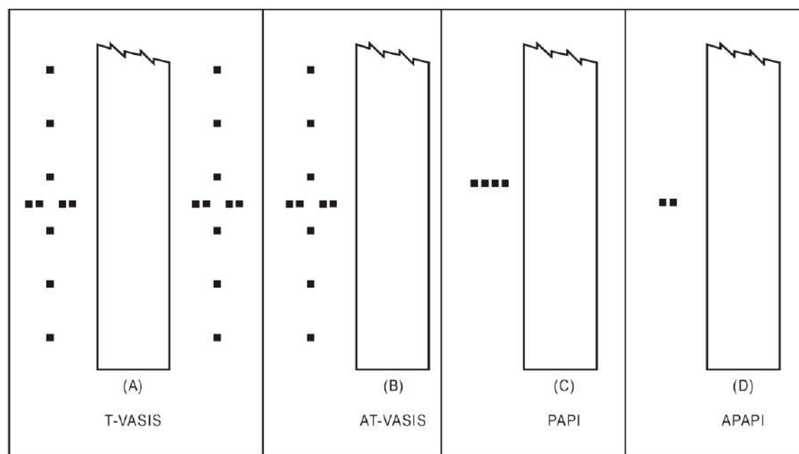
Figure 5-16. Visual Approach Slope Indicator Systems
