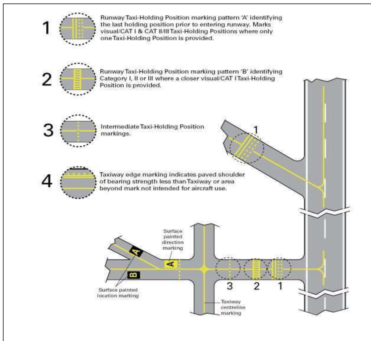
Figure 5-6 Taxiway markings
